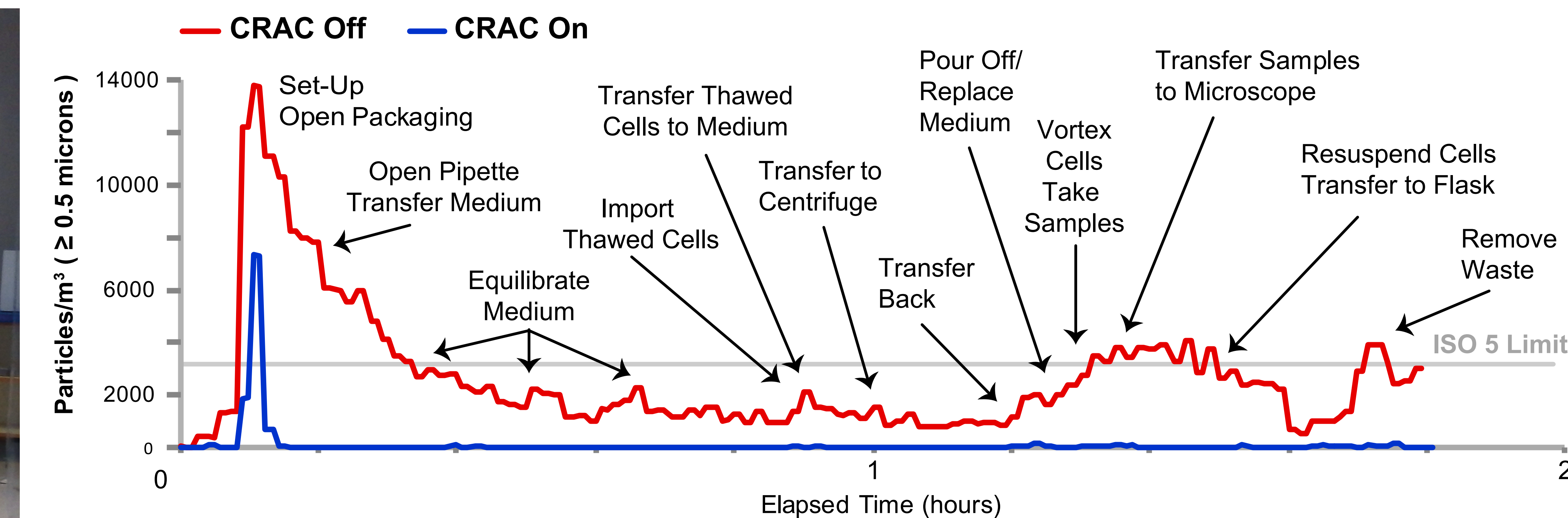
Figure 2. The CRAC System Controls Airborne Particles During a Routine Cell Thawing Process. A routine cell thawing process was performed with the Continuously Recirculating Air Cleaning (CRAC) System on or off. The CRAC rapidly removed particles from the Processing Chamber Air that otherwise would have remained aloft.
